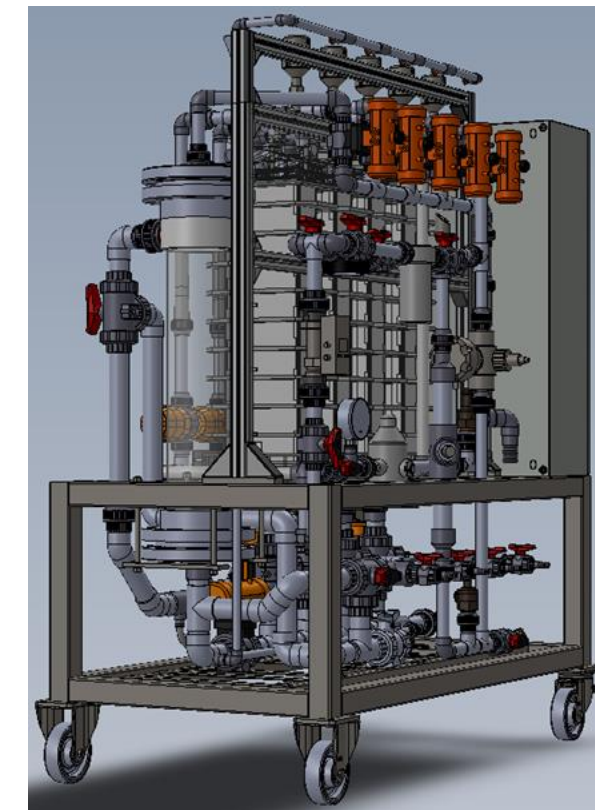
Design of the pilot plant
